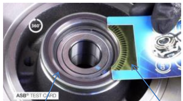
ASB®-Magnetencodier
