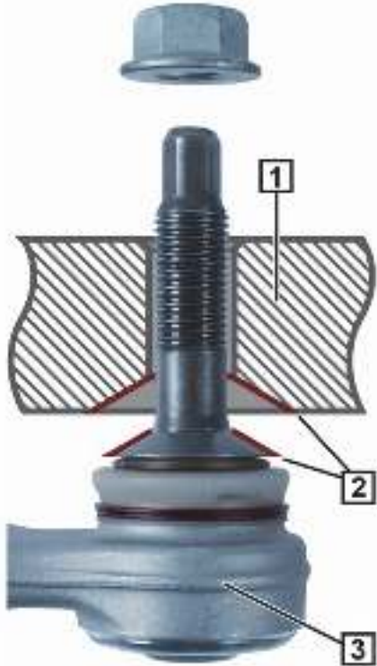
Fig.1: Rear axle control with cone seat (2)
